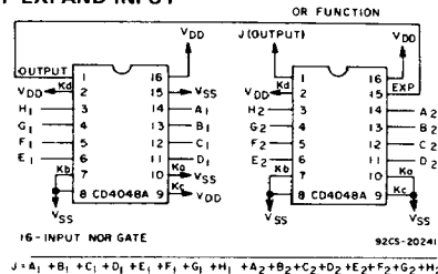
Fig. 5 - 16-input NOR gate.
