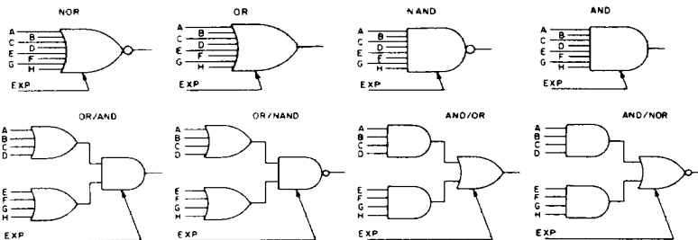
Fig. 1 - Basic logic configurations.
